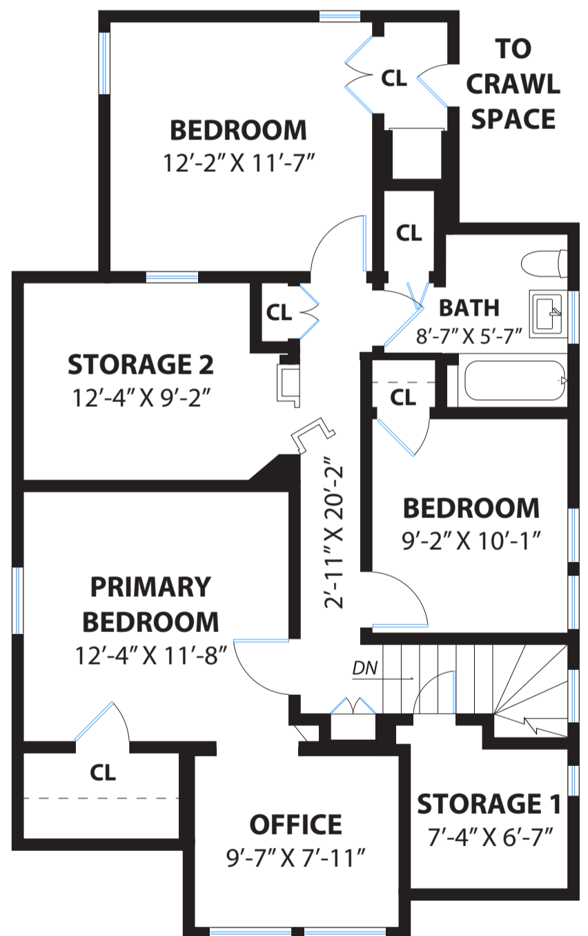
UPPER LEVEL
