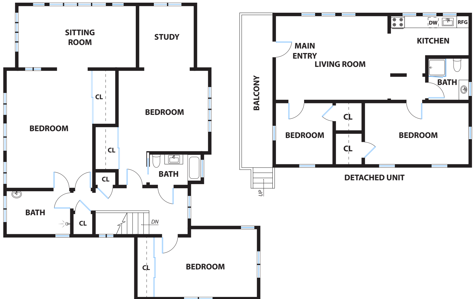
UPPER LEVEL
