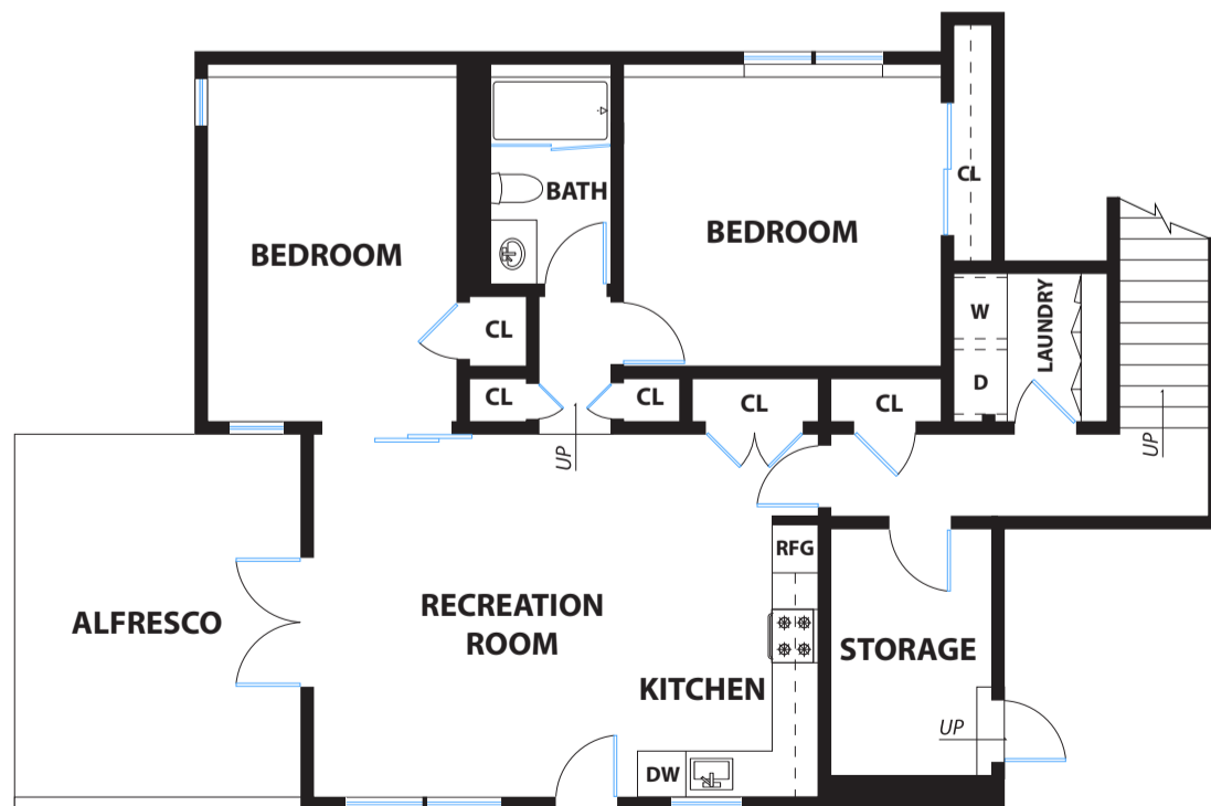
LOWER FLOOR
